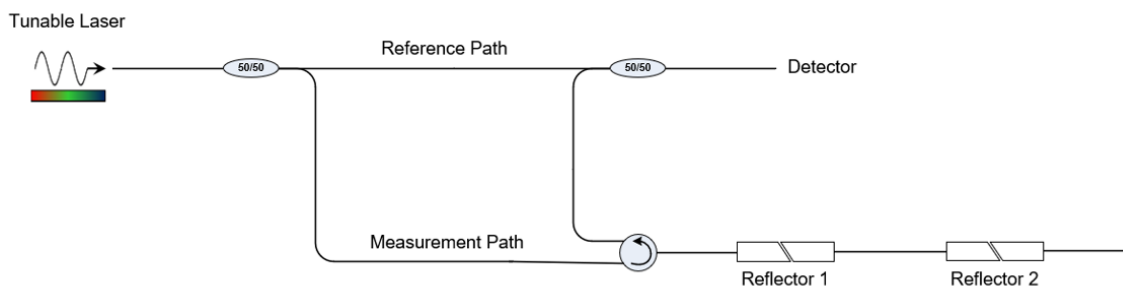
Figure 309 Basic OFDR Optical Network with two partial reflectors (connectors)
