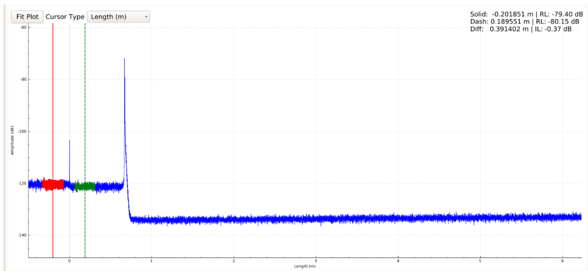
Figure 104 Insertion loss measurement shown across an APC fiber connector. (IL is shown in upper right corner)
